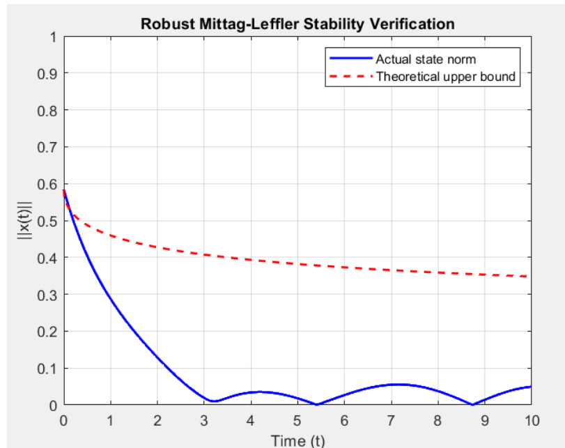
Figure 1. State trajectories with state-dependent delay of Example 4.1.
