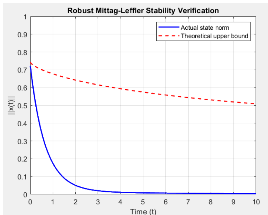
Figure 2. State trajectories with state-dependent delay of Example 4.2.
