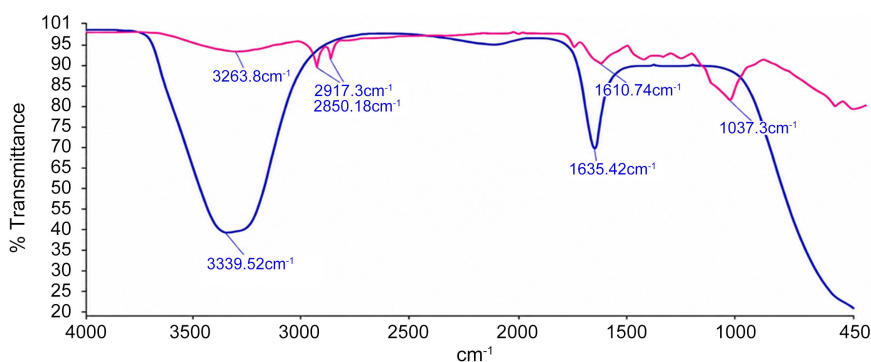
Figure 2. FTIR of Justicia carnea dye extract (blue colour represents water, medium of extraction while red colour represents dye extract).
