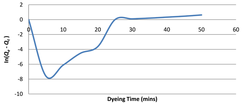
Figure 6. Graph of pseudo-first order adsorption kinetics of J. carnea dyes on pre-mordanted cotton fabric sample.
