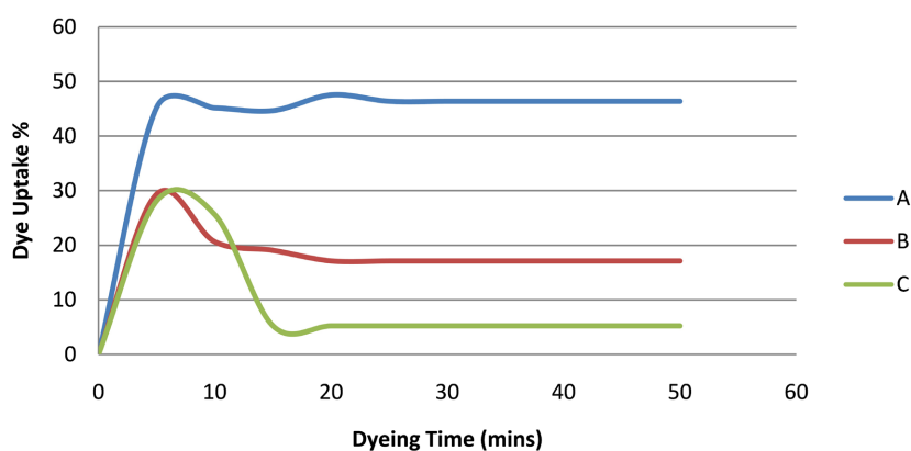
Figure 4. Effect of Time and Temperature on J. carnea dye adsorption on Mordanted Cotton Sample A (50°C), B (60°C) and C (70°C).
