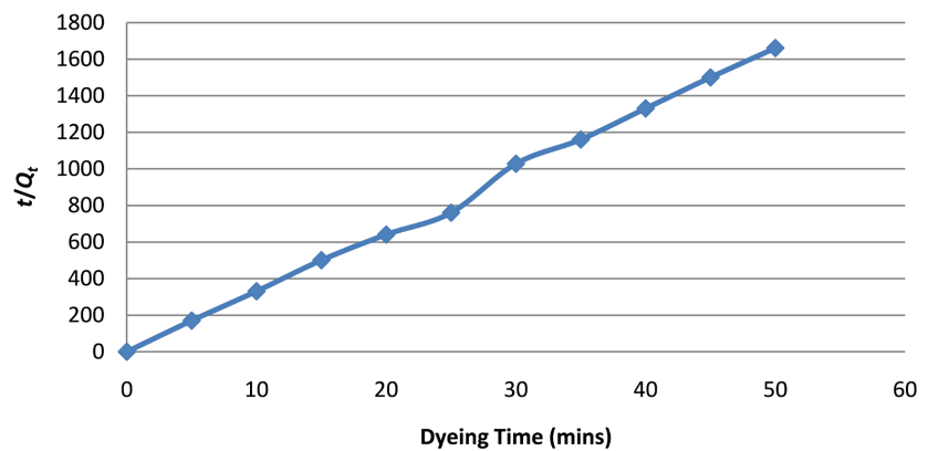
Figure 7. Graph of pseudo-second order adsorption kinetics of Justicia carnea dyes on unmordanted cotton fabric sample.
