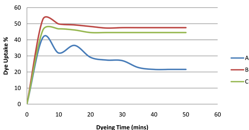
Figure 3. Effect of time and temperature on J. carnea dye adsorption on un-mordanted cotton fabric A (50°C), B (60°C) and C (70°C).
