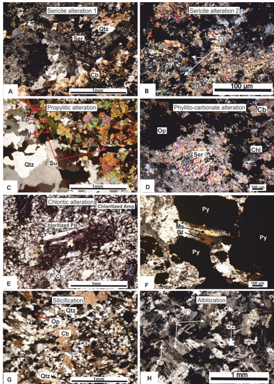
Figure 4. Microscopic view of altered rocks from Diénéméra-Gongondy copper deposits. Sericitic alteration 1 (A), Sericitic alteration 2 (B), Propylitic alteration (C), Phylitic-carbonate alteration (D), Chloritic alteration (E), Residual potassic alteration (F), Silicification (G) and Albitization (H). Minerals abbreviations: Amp: Amphibole, Bt: biotite, Cb: carbonate, Chl: chlorite, Ep: epidote, Ms: muscovite, Op: Opaques, Pl: plagioclase, Py: pyrite, Qtz: quartz, Ser: sericite, Sulf: sulfides.
