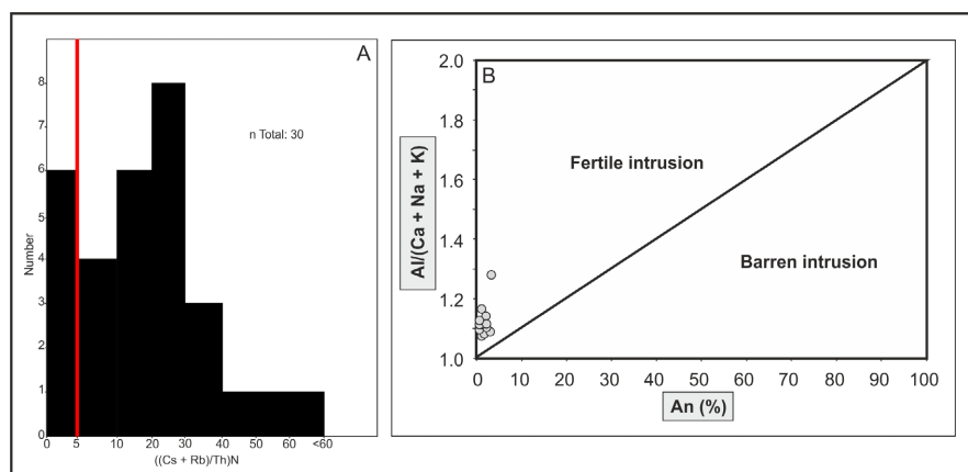
Figure 11. Graph of potential mineralisation index using the primitive mantle normalized formula of [47]. The red line corresponds to limit of potential mineralization which must be more than 5 units (A). Binary diagram of [66] for the determination of the fertility of intrusions. Most of the samples fell in the fertile intrusion field (B).
