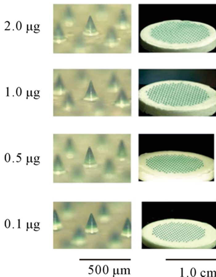
Dissolving microneedles and their array chips containing 0.1 - 2.0 µg bFGF. The tip portion where bFGF was formulated was stained with brilliant blue.
