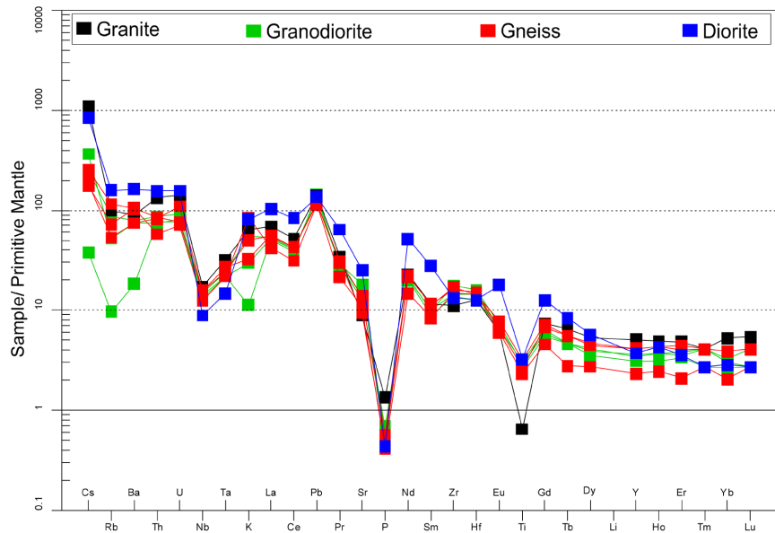
Figure 5. Primitive mantle-normalized multi-element spider diagrams for the Zoukougbeu studied rocks (Primitive mantle values from [21]).
