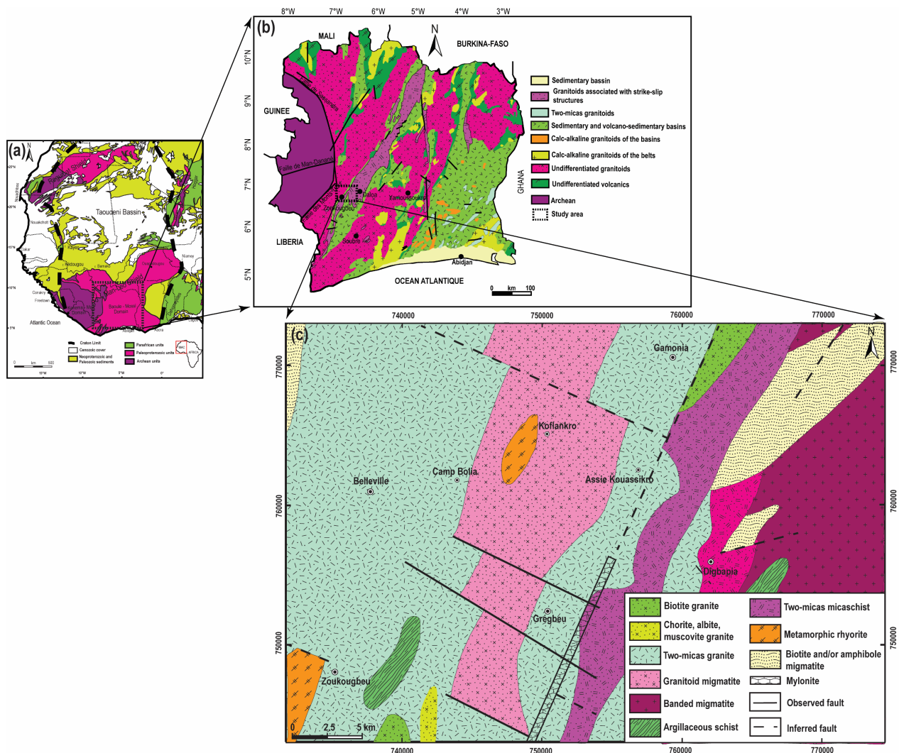
Figure 1. (a) Geological map of the West African Craton showing the location of the Ivory Coast (modified after [13]). (b) Simplified geological map of the Ivory Coast (modified after [14]). (c) Geological map of the Zoukougbeu area (modified after [15]).
