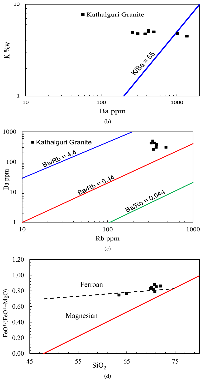
Figure 18. (a) The K vs. Rb diagram after Taylor, 1965 [30] for Kathalguri Granite. (b) The K vs Ba diagram after Mason 1966 [32] for Kathalguri Granite. (c) Rb vs Ba plot after Mason 1966 [32] for Kathalguri Granite. (d) Chemical classification of Kathalguri Granites using \text{FeO}^*/(\text{FeO} + \text{MgO}) vs \text{SiO}_2 diagram after Frost et al. (2001) [28].
