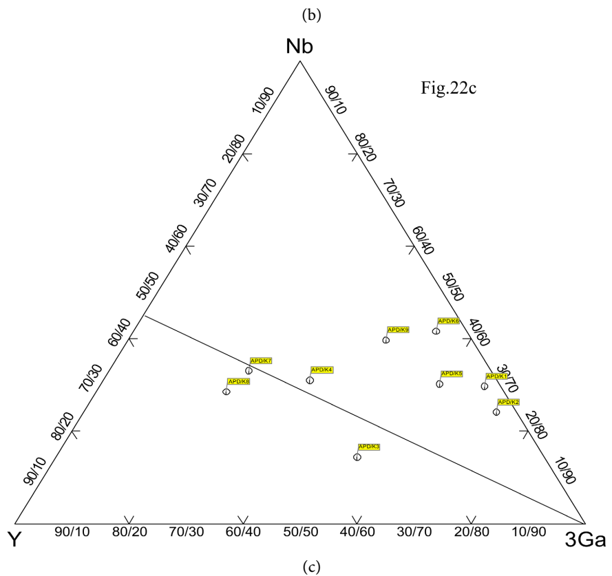
Figure 22. Ternary plots after Eby 1992 [41] for Kathalguri Granite occupying A1 type granite ( n = 6 Samples while (Truly Anorogenic Rifting), and only two samples plot (APD/K/3 and APD/K/8) in A2 type (Post-Collisional) field. (a) \text{Fe}_2\text{O}_3^*5 - (\text{Na}_2\text{O} + \text{K}_2\text{O}) - [(\text{CaO} + \text{MgO})^*5] , (b) Ce-Y-Nb and (c) 3Ga-Y-Nb plot.
