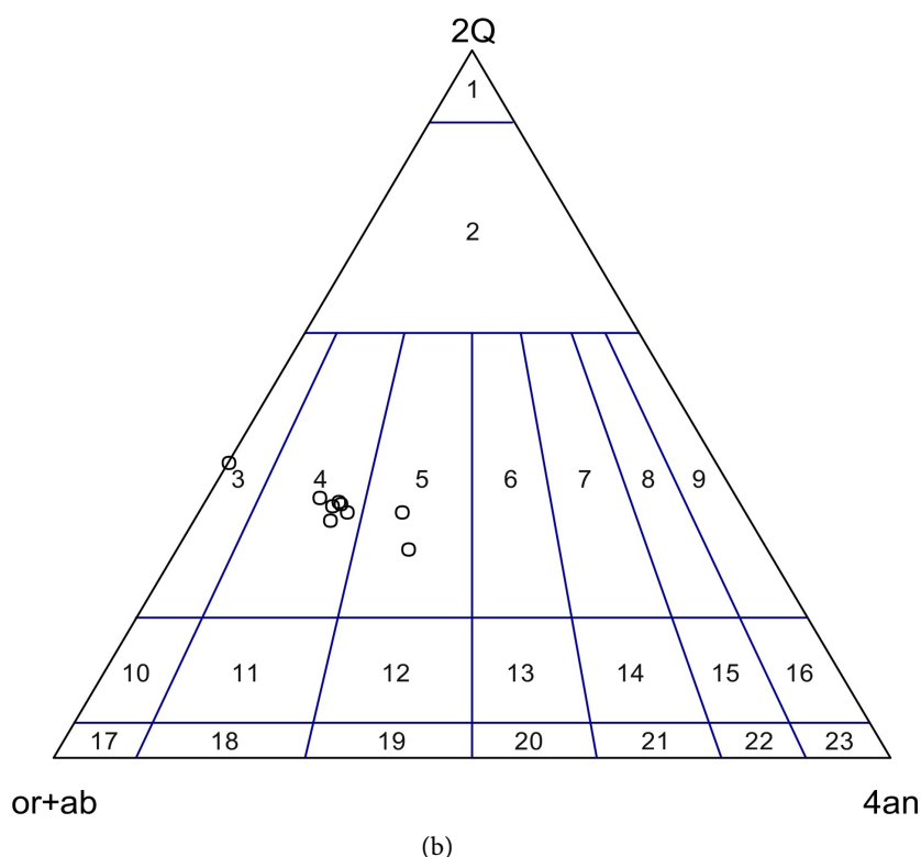
Figure 13. (a) Modal QAP Diagram after Strieckessens (1976) [20] for Kathalguri Granite. Fields. 0 Quartzolite, 1 Quartz rich Granitoid, 2 Alkali Feldspar Granite, 3a SNG Syeno-Granite, 3b MZG Monzo-Granite, 4 Granodiorite, 5 Tonalite, 6 Quartz alkali feldspar Syenite, 7 Quartz Syenite, 8 Quartz Monzonite, 9 Monzodiorite Monzogabbro, 10 Quartz Diorite Quartz Gabbro, Quartz Anorthosite, 11 Alkali Feldsapr Syenite, 12 Syenite, 13 Monzonite, 14 Foid bearing Monzo diorite monzo gabbro, 15 Diorite, Gabbro Anorthosite. (b) Normative (Or + Ab) - 2Q - 4An Ternary plot for Kathalguri Granite occupying Syeno-Granite ( n = 7 ) to Monzogranite Field ( n = 2 ) after Enriques 2018 [21]. 1 quartzolite, 2 quartz-rich granitoids, 3 al kali-feldspar granite, 4 syenogranite + sub-anorthite monzogranite, 5 monzogranite, 6 granodiorite, 7 tonalite, 8 tonalgabbro, 9 tonaleu crite, 10 quartz alkali-feldspar syenite, 11 quartz syenite, 12 quartz monzonite, 13 quartz monzodiorite/quartz monzogabbro, 14 quartz diorite, 15 quartz gabbro, 16 quartz eucrite, 17 alkali feldspar syenite, 18 syenite, 19 monzonite, 20 monzodiorite/monzogabbro, 21 diorite, 22 gabbro, 23 eucrite.
