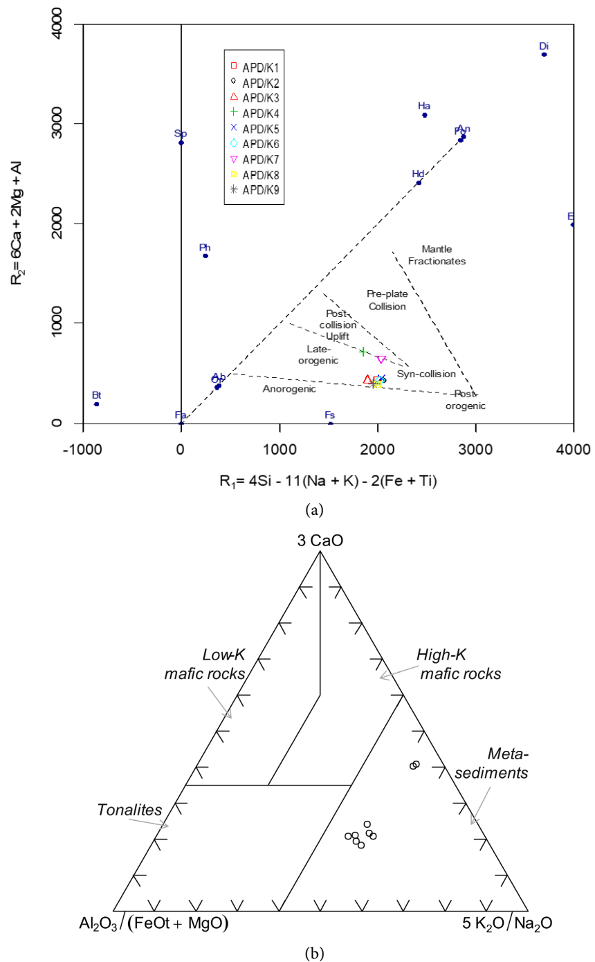
Figure 19. (a) R1-R2 plot after Batchelor and Bowden 1985 [33] for Kathalguri Granite. (b) Source diagram after Laurent et al. 2014 [34] for Kathalguri Granite showing its source by metasediments.
