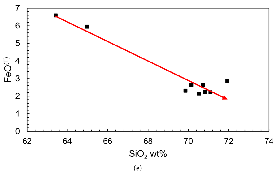
Figure 27. (a) Ba vs Eu plot. (b) La vs (La/Yb) N plot. (c) Rb vs Rb/Nd plot. (d) Rb/V vs Rb plot showing Mixing and Fractional crystallization trends after Schiano et al. (2010) [60]. (e) SiO 2 vs FeO (T) plot showing negative correlation indicates fractionation of feldspar and Fe-Ti oxides.
