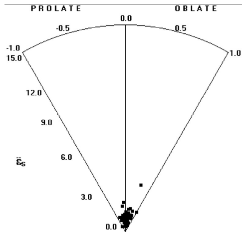
Figure 10. Hsu diagram [16] with Flinn's k-values for pebbles of Mikir Hills, represents an intermediate zone between pure flattening and pure constriction.
