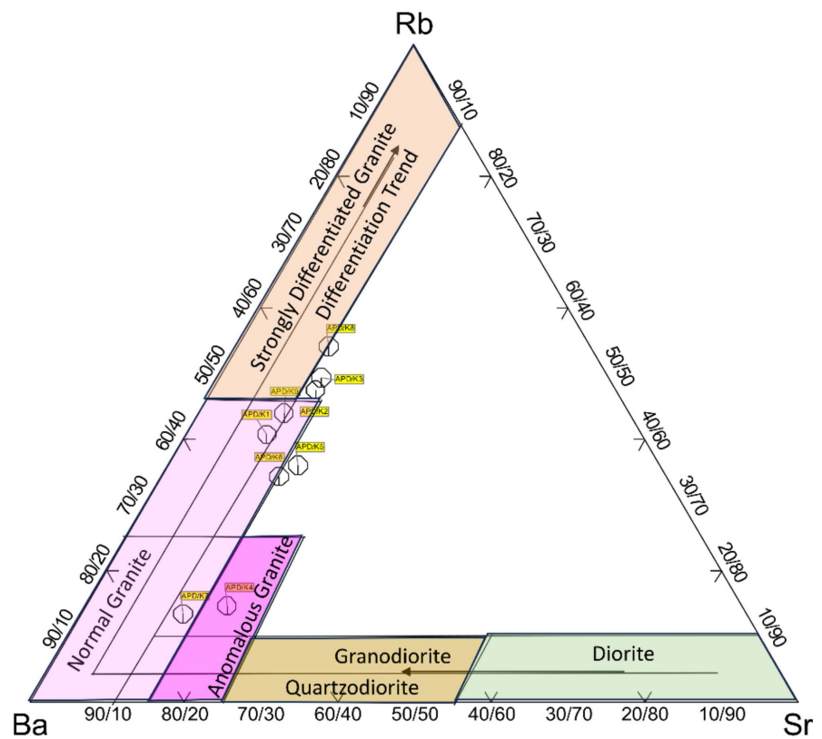
Figure 24. Rb-Ba-Sr ternary diagram after El Bouseily and El Sokkary 1975 [55] for Kathalguri Granite showing Anomalous-normal to strongly differentiated type of granite.
