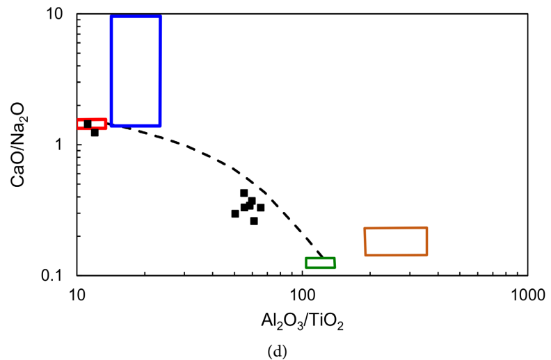
Figure 26. Chemical discrimination diagrams illustrating the mineral fractionation process for the Kathalguri Granite. (a) Rb versus Sr, (b) Ba versus Sr Abbreviations: Bt, Biotite; Ms, Muscovite; Cpx, clinopyroxene; Hbl, hornblende; Kfs, K-feldspars; Plg, plagioclase; Amph, Amphibole, Grt, Garnet. Plots after Sylvester 1998, Wu et al. 2017 [58] [59]. (c) Cr vs Ni Plot for Kathalguri Granite showing fractionation trend. (d) Kathalguri Granite in \text{CaO}/\text{Na}_2\text{O} vs \text{Al}_2\text{O}_3/\text{TiO}_2 plot. The “MORB” (red rectangle) composition is compiled from GERM database http://earthref.org/ , and “Pelite-derived melt” (green rectangle) field is from Patiño Douce and Johnston (1991) [61]. The compositions of the eclogitic amphibolites (blue rectangle) likely part of the lower plate involved in the Variscan collision (Medaris et al. 2003) [62], and the average composition of country-rock metasediments (orange rectangle). Kathalguri Granite showing enriched mantle-derived and crustally-derived melts by occupying compositional field in between MORB to Pelite-derived melt position.
