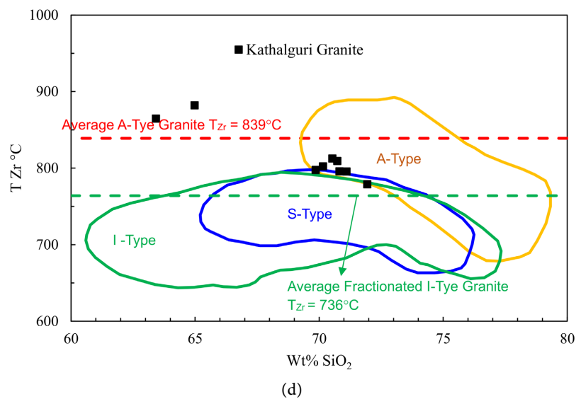
Figure 28. (a) Zircon Saturation Temperature vs Zr plot. (b) T Zr vs Zr plots with M fences. (c) SiO 2 vs Zr plot showing negative correlation. (d) SiO 2 vs T Zr plot for Kathalguri Granite showing it's a type characteristic.
