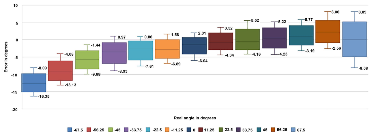
Figure 10. Representation of angular errors versus actual angles in the anechoic chamber.
