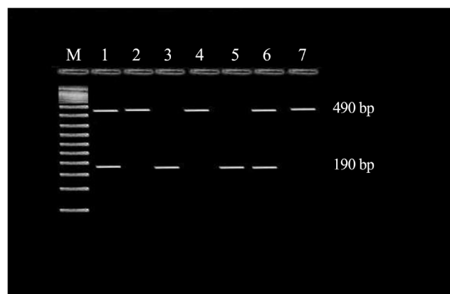
Figure 1. Detection of genetic polymorphism of ACE using PCR amplification: This figure showed 3 main different picture (DD, ID and II): DD homozygous (a single 190 base pair), ID heterozygous (190 and 490) Base pair, II homozygous (490 bp).
