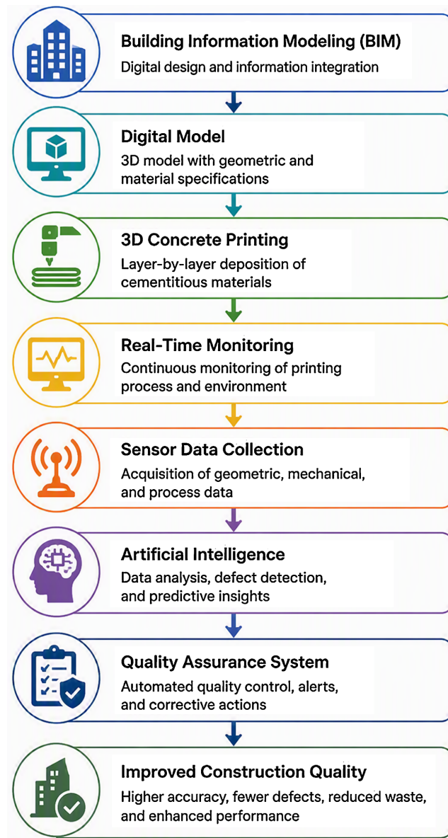
Figure 1. Conceptual framework for quality control in 3D concrete printing.
