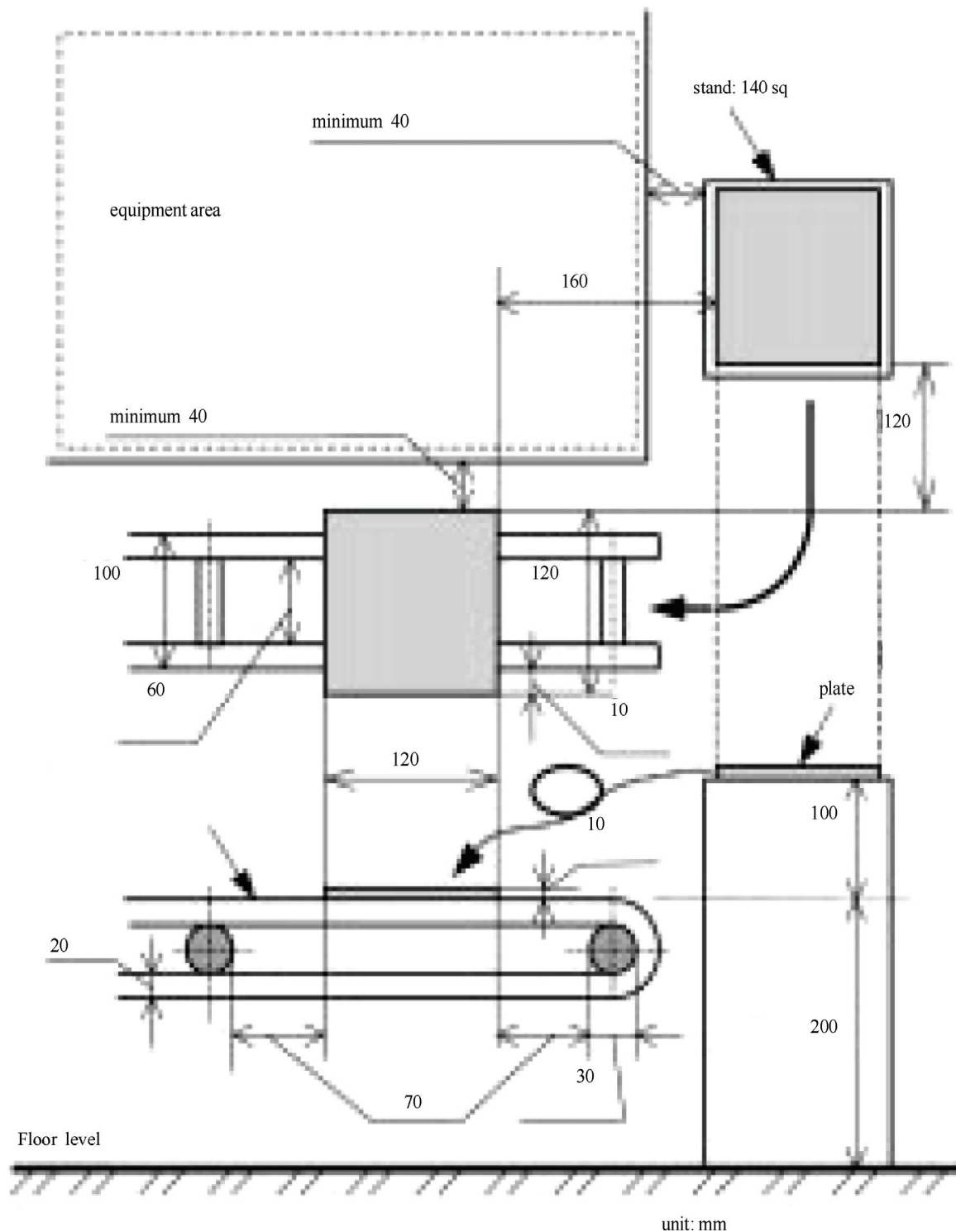
Figure 1. 1997 street artist robot competition (frog-like machine blowing soap bubbles).
