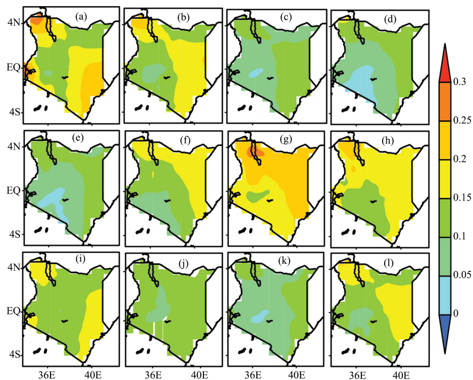
Figure 3. Annual spatial variation of Aerosol Optical Depth (AOD) using MERRA-2 Model data during 20001-2024 period.
