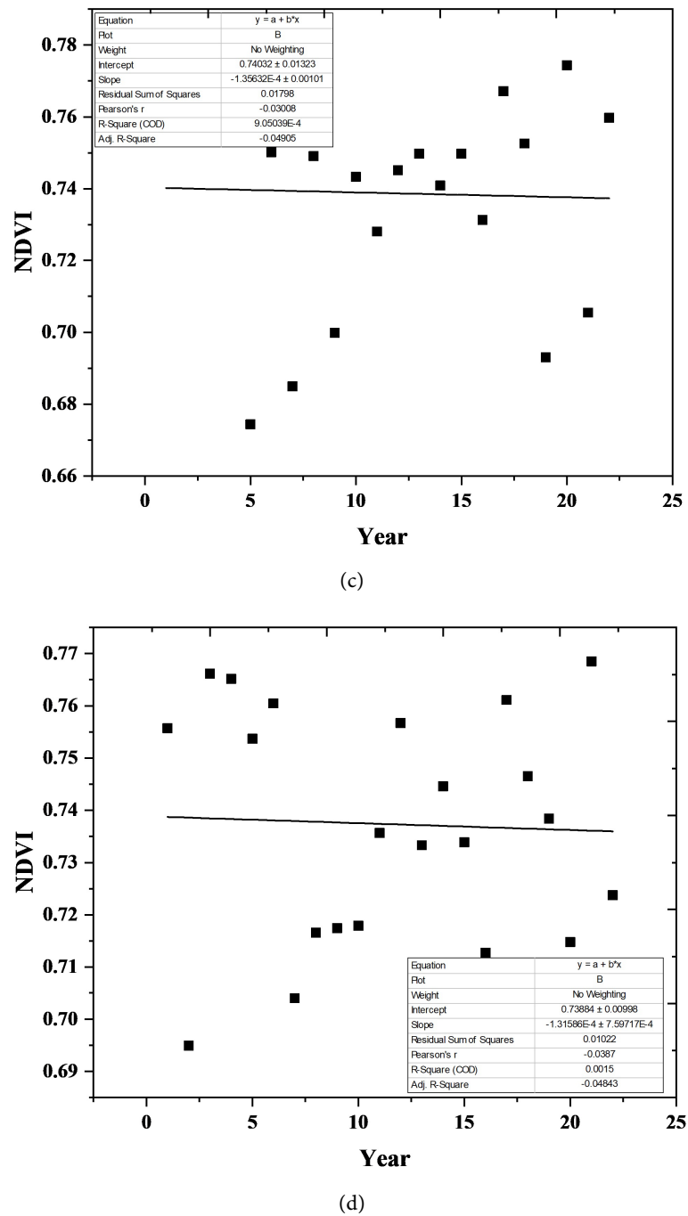
Figure 2. Seasonal trend of NDVI over Mau Forest complex.
