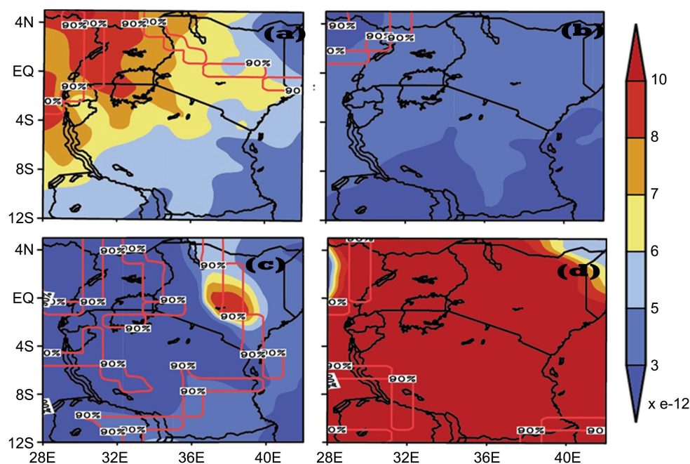
Figure 4. Seasonal spatial variation of BC Surface Mass Concentration using (a) JF, (b) MAM, (c) JJAS and (d) OND seasons over EA during 1980-2023.
