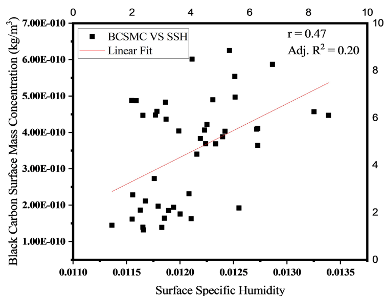
Figure 6. Seasonal correlation between BC Surface Mass Concentration and Surface Specific Humidity averages using (a) DJF, (b) MAM, (c) JJAS and (d) SON seasons over EA during 1980–2023.
